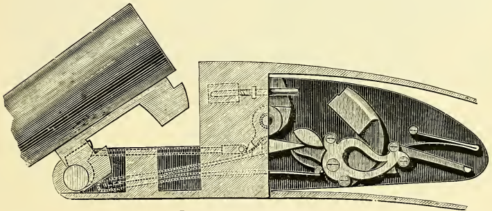
Purdey's Hammerless Gun.
